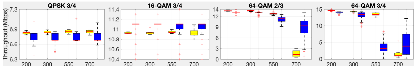
Fig. 10. Values of network throughput for different MCSs for different MCSs, as a function of the distance between RSU and OBU. Results refer to the rural scenario (Fig. 7 – C). Each boxplot pair is: 1) VEINS-HP; 2) Trials-HP.
