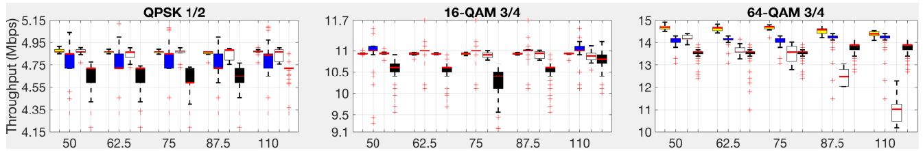
Fig. 8. Values of network throughput for different MCSs, as a function of the distance between RSU and OBU. Results refer the urban scenario (Fig. 7 – A). Each quartet represents the results for a single position with the order (from left to right): 1) VEINS-HP; 2) Trials-HP; 3) VEINS-LP; 4) Trials-LP.
