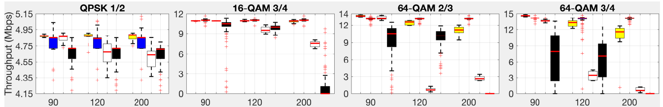
Fig. 9. Values of network throughput for different MCSs for different MCSs, as a function of the distance between RSU and OBU. Results refer to the suburban scenario (Fig. 7 – B). Each quartet follows the same order as in Fig. 8.
